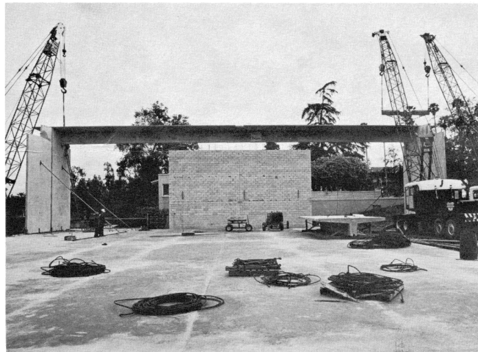
CONSTRUCTION PROGRESSES—Large cranes lift first mammoth roof beam—116 feet long and 54 tons—into place. Left, 38,000-pound wall panel of prestressed concrete is bolted in position.
